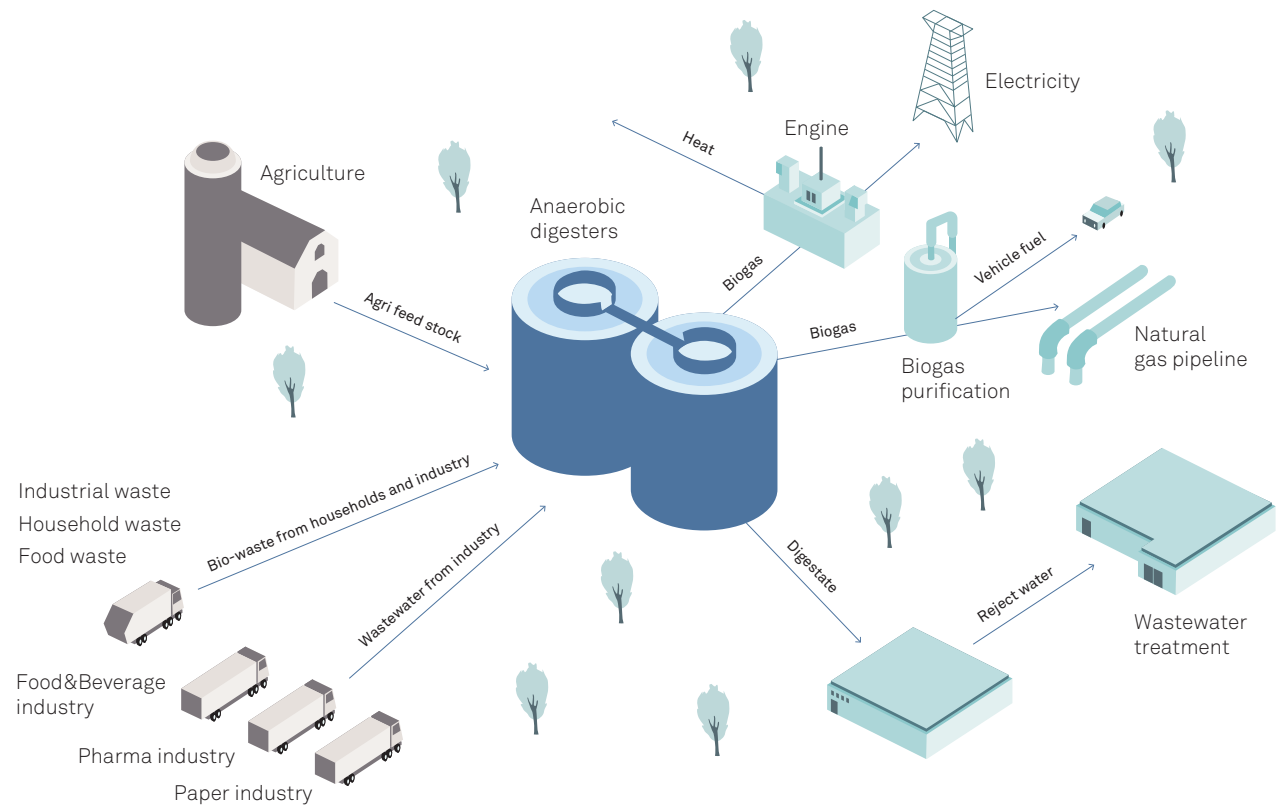
Figure 6.2 Schematic picture over a biogas plant showing the utilization of substrates and biogas.
